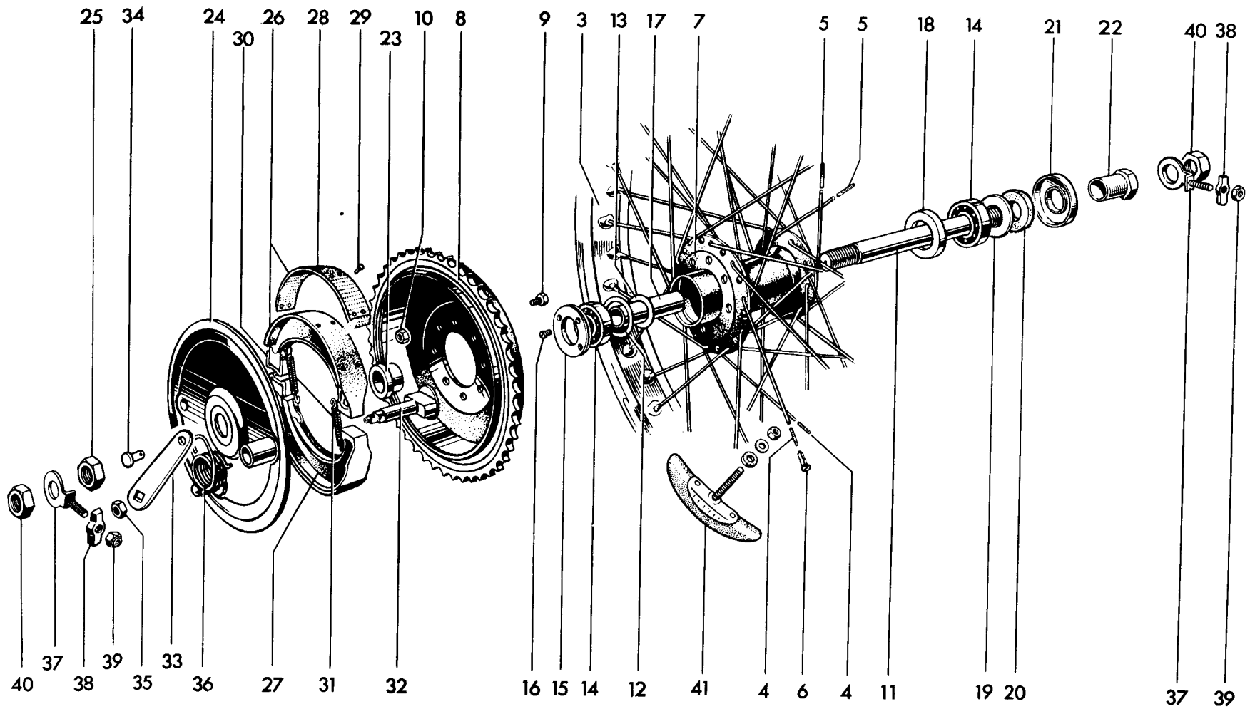
Fig. 20. REAR WHEEL
