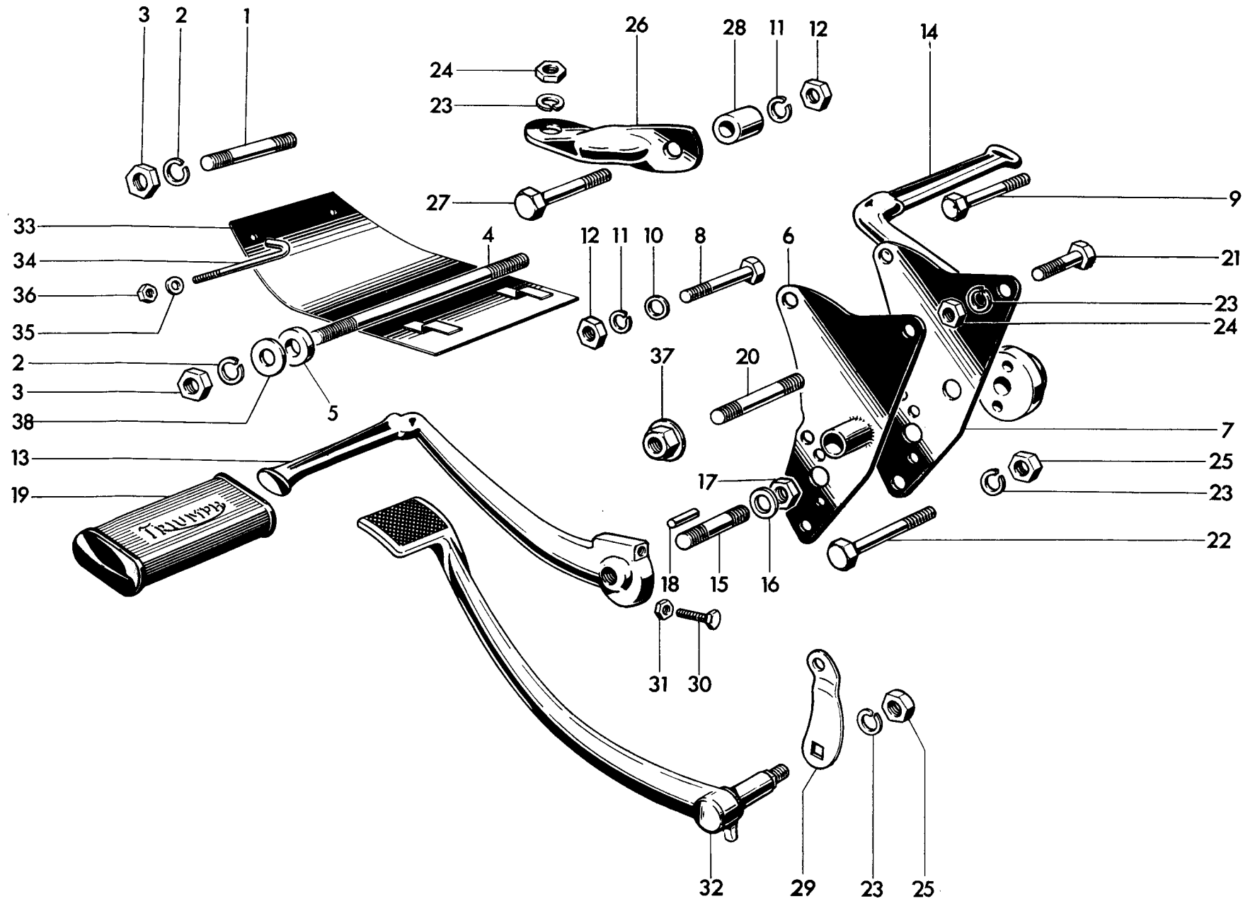
Fig. 14. ENGINE UNIT FITTINGS AND FOOTRESTS
