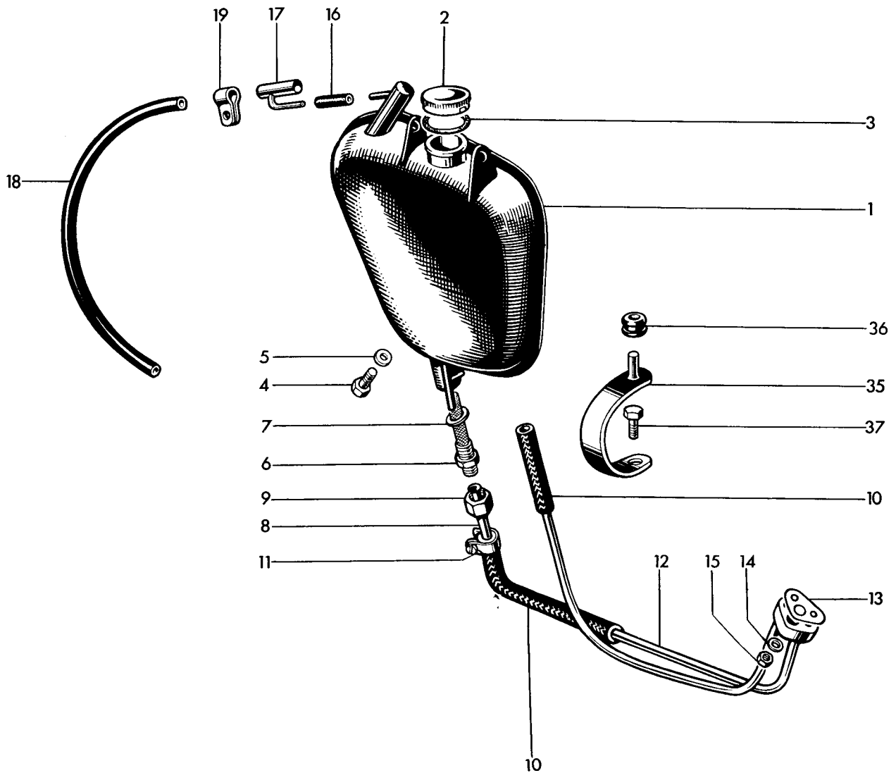
Fig. 23. OIL TANK
