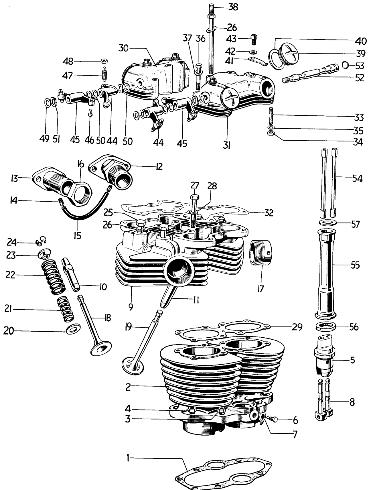
Fig. 5. CYLINDER BLOCK AND HEAD, T120
