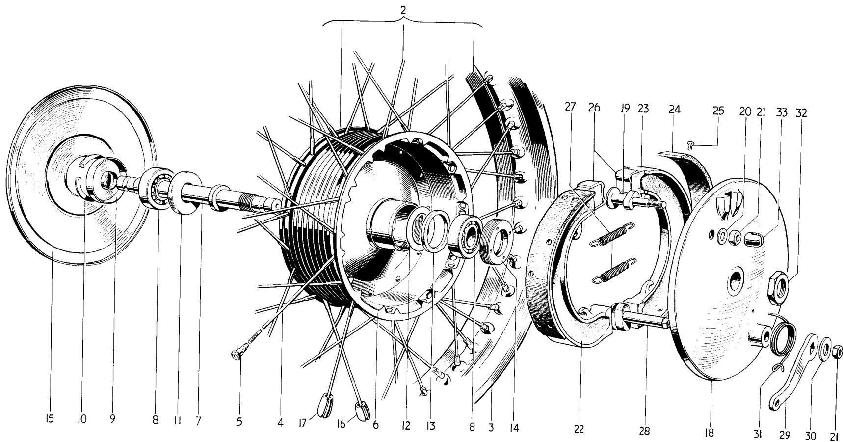
Fig. 19. FRONT WHEEL
